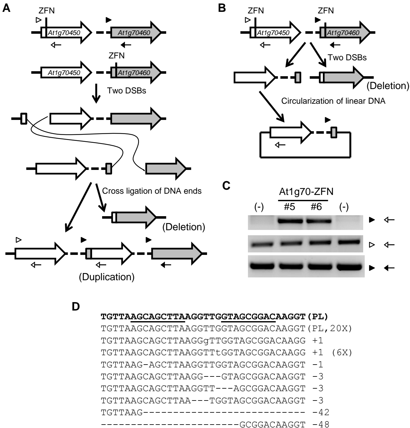
Figure S9 Duplication of a gene cluster or circularization of deleted DNA at the At1g70450 - At1g70460 locus. (A) Schematic of the At1g70450 gene cluster duplication. (B) Schematic of circularization of deleted DNA. (C) PCR confirmation of possible gene cluster duplications. (D) DNA sequence data from clones indicative of possible gene cluster duplications.
