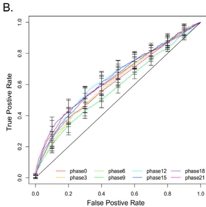
Figure S5 Precision-recall and AUC-ROC curves of SVM predictions for C. reinhardtii . (A) Precision-recall curves for the prediction of each of the eight phase clusters in cycling genes in C. reinhardtii as classified using SVM. Each phase-cluster is represented as a different colored line: 0 (red), 3 (orange), 6 (lime), 9 (green), 12 (teal), 15 (blue), 18 (purple), 21 (pink). Error bars represent the variance in 10 separate runs of the SVM classifier at optimal parameters. (B) ROC curves for the prediction of each of the eight phase clusters in cycling genes in C. reinhardtii as classified using SVM. Line color and error bars are assigned as in (A).
