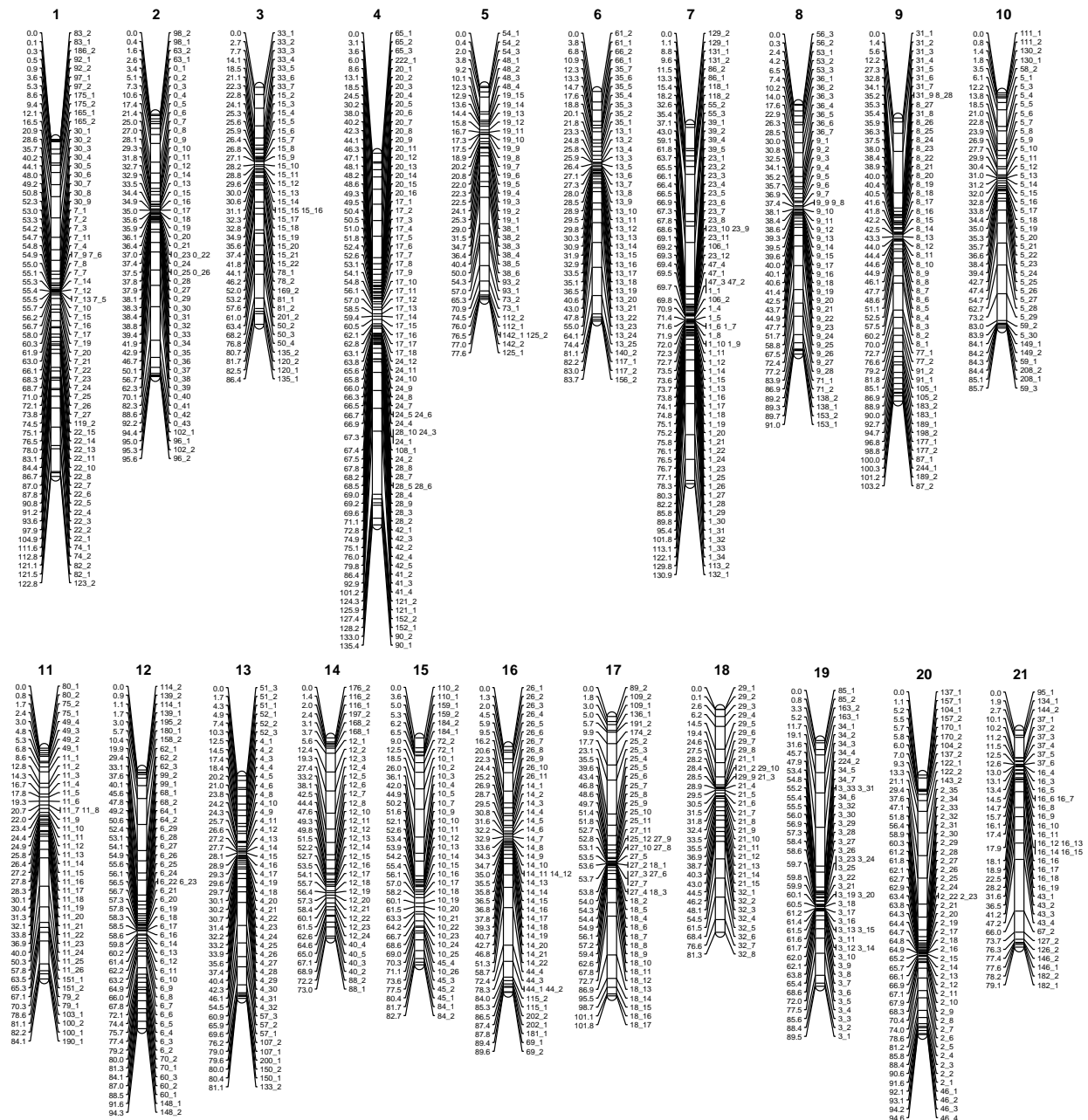
Figure S4 Linkage map from BEPA x LITC cross
