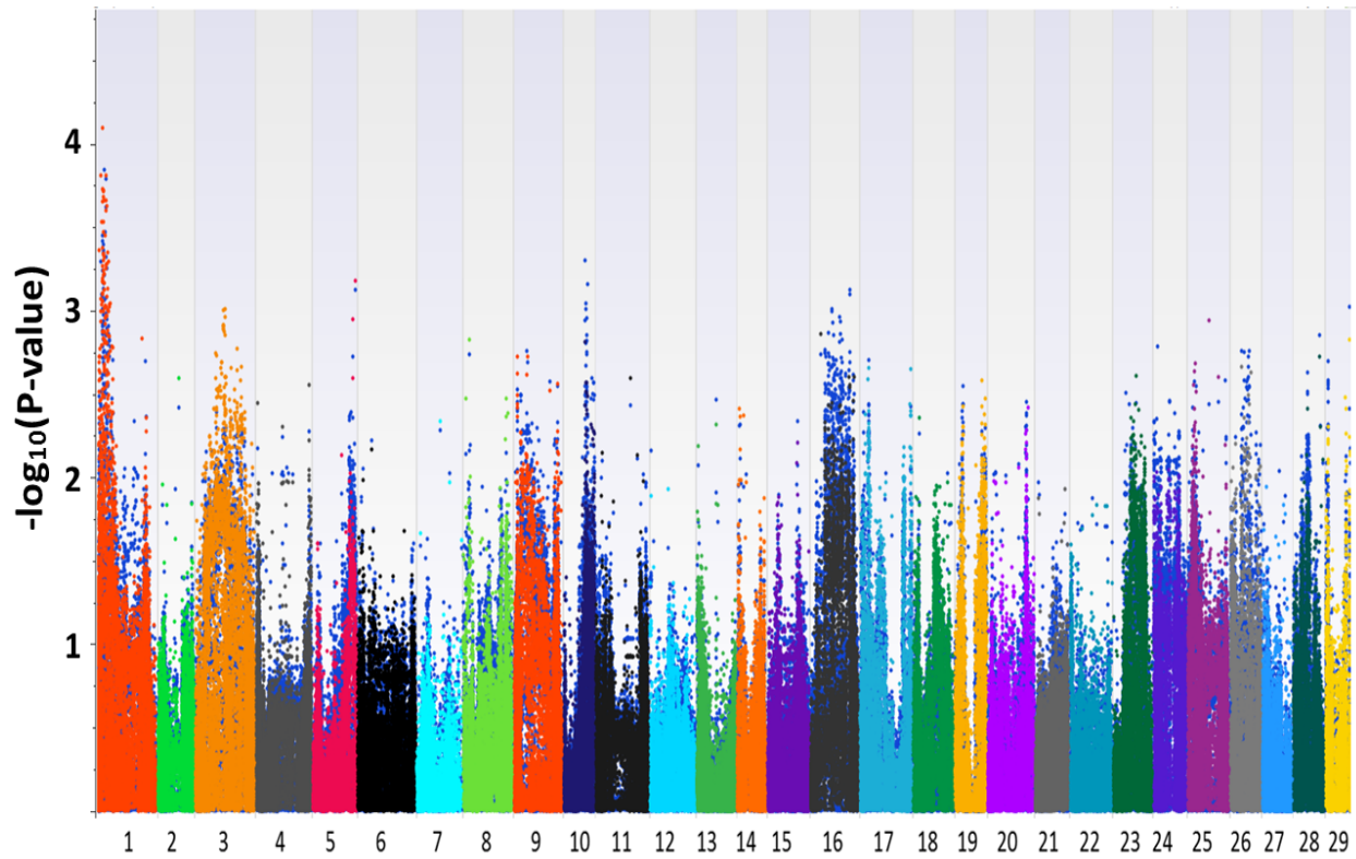
Figure S5. Manhattan plots for head depth. The plots in different colors in the front layer were generated from EMMAX and the plots in blue in the back layer were generated from QFAM.
