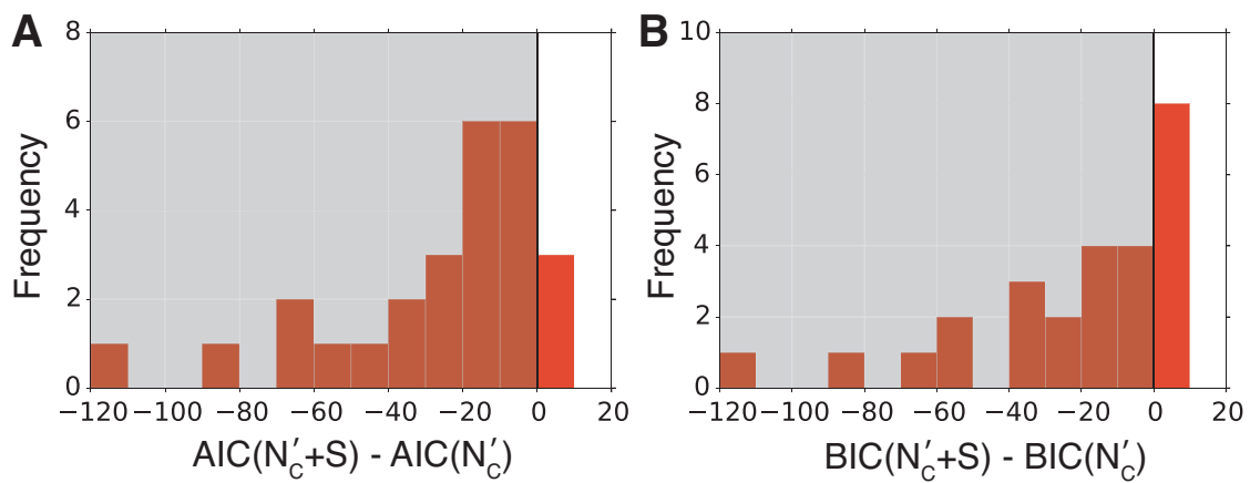
Figure S1: Inclusion of the aSD binding strength score, S , to multivariate regression between protein abundance and codon usage bias ( N'_c ) enhances total predictive power of multiple regression models as evidenced by lower (A) AIC and (B) BIC scores.
