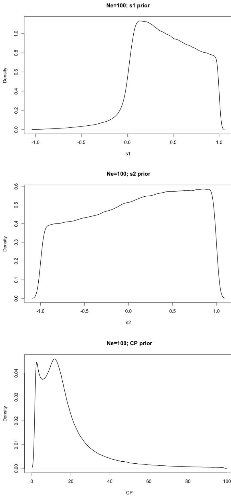
Figure S1. Updated prior distributions of s1 , s2 , CP for a haploid population with N_e=100 after the constraint of trajectories segregating at change point.
