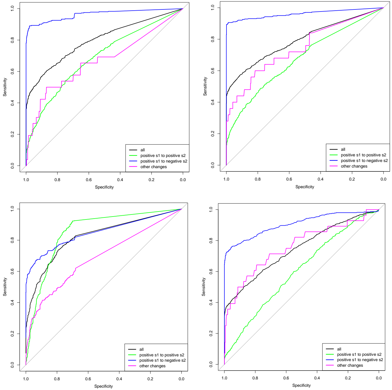
Figure S3. ROC curves of the Bayes factor B_{0,1} from the ABC model choice of a haploid population with N_e=[1000,10000] (above) and a diploid population with N_e=[50,5000] (below).
