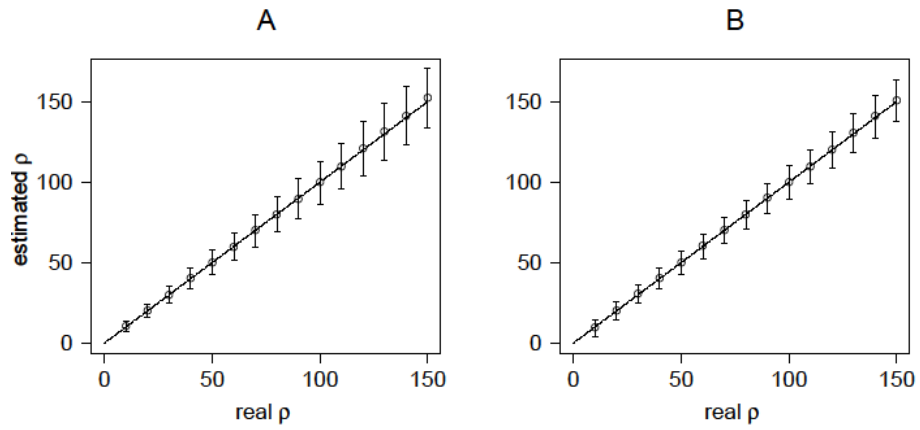
Figure S3 Comparisons of \rho_{FastEPRR} when the sample size is very large ( n = 1000 ). The mean and the standard deviation of \hat{\rho} was estimated from 2,000 simulated data conditional on \rho and S = 75 (A) or 375 (B).
