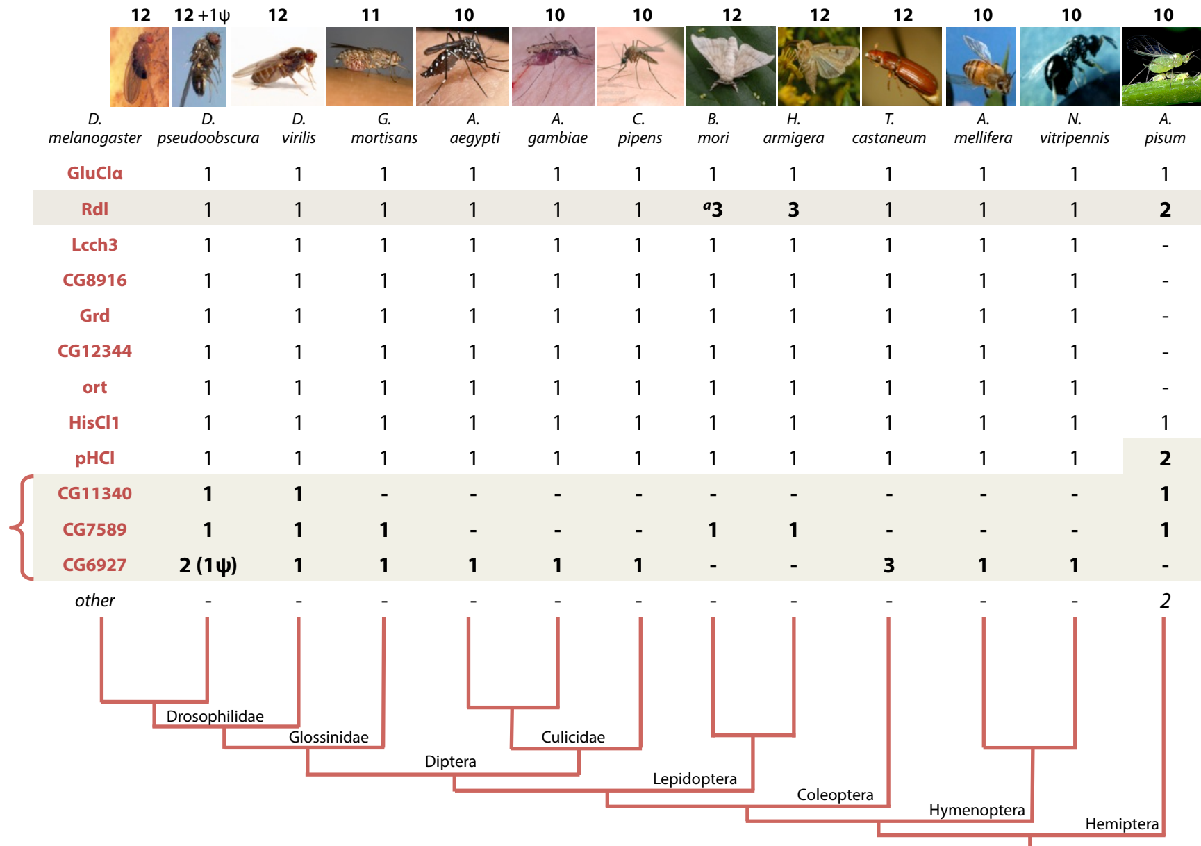
Figure S1. LGCC gene copy number present in the genome sequences of insect species. Total number of subunits in each species is indicated at the top of the figure. Orthologues are compared to the D. melanogaster reference gene set. Copy number was determined by BLAST searches.
