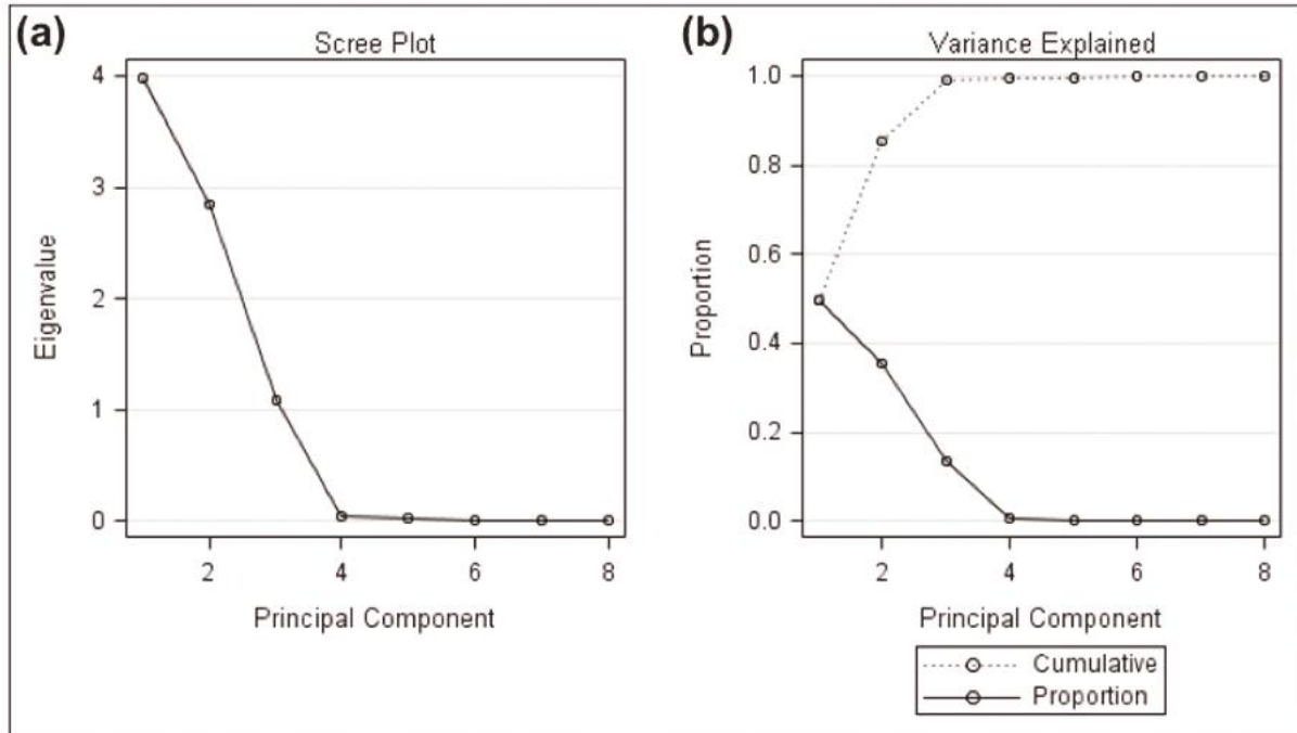
Figure S1. Principal component analysis of kernel weight and shape traits. (a) Eigenvalues of principal components (PCs). PCs with eigenvalue greater than 1 were retained. (b) Variance explained by different PCs. Dashed line represents the cumulative variance, while solid line represents variance explained by single PC
