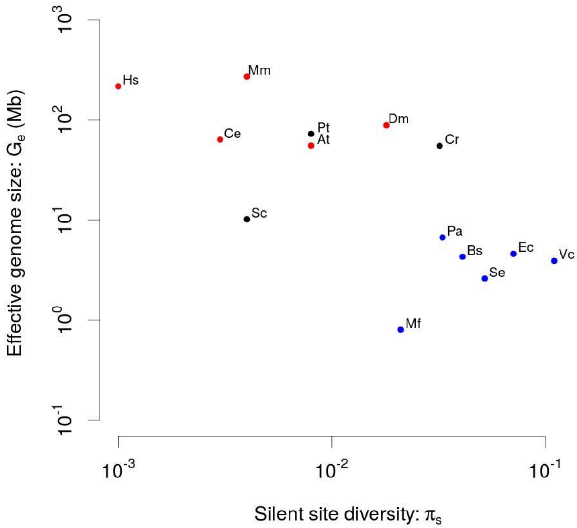
Figure S6: A scatter-plot of effective genome size ( G_e ) against silent site diversity ( \pi_s ).
