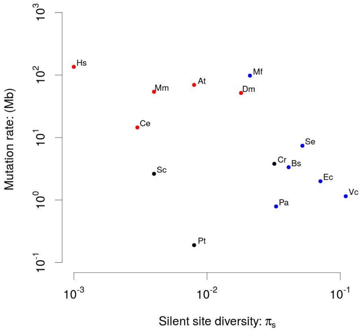
Figure S7: A scatter-plot of base-substitution mutation rate ( u_{bs} ) against silent site diversity ( \pi_s ).
