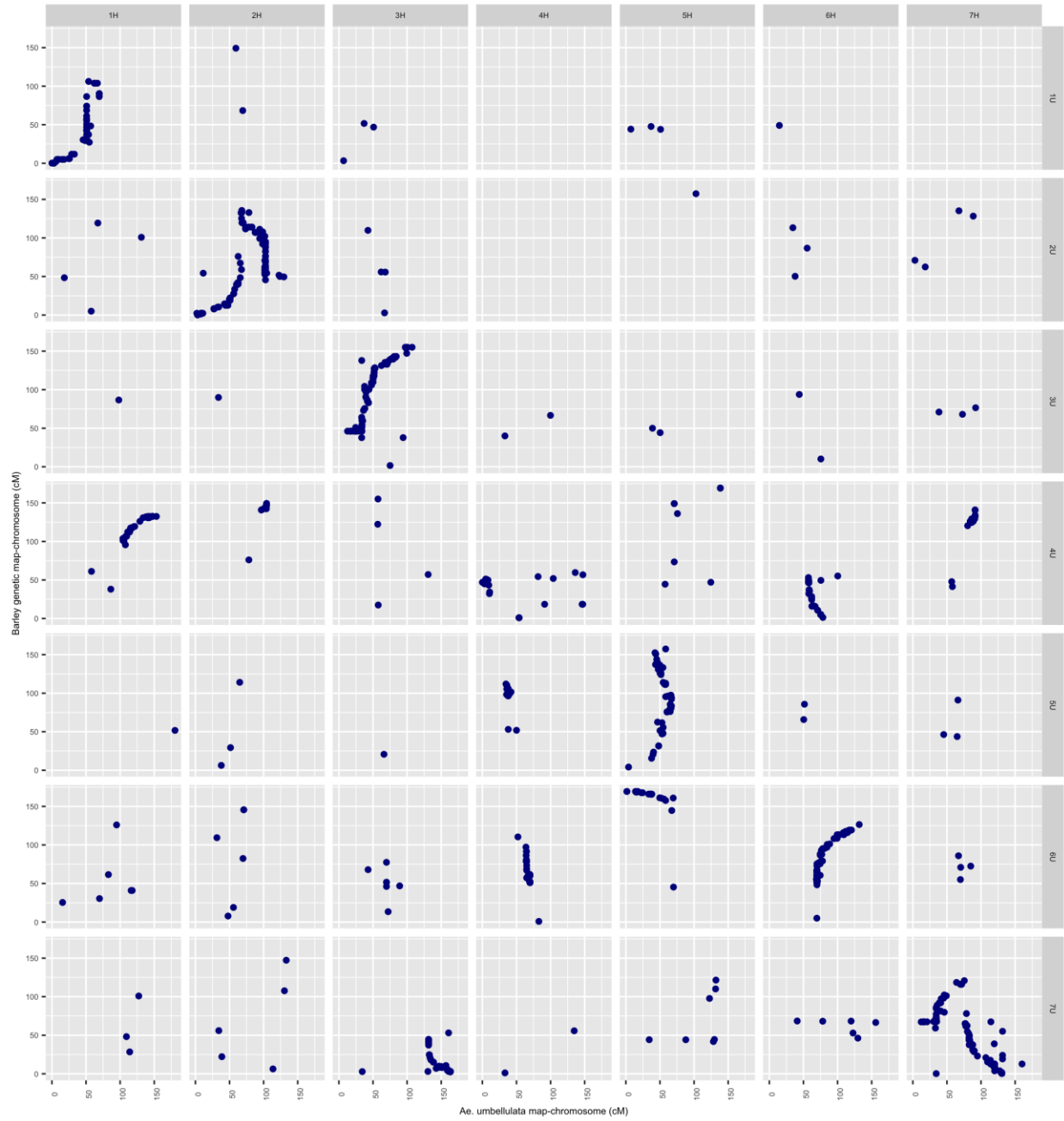
Marker order comparison - Ae. umbellulata vs barley
