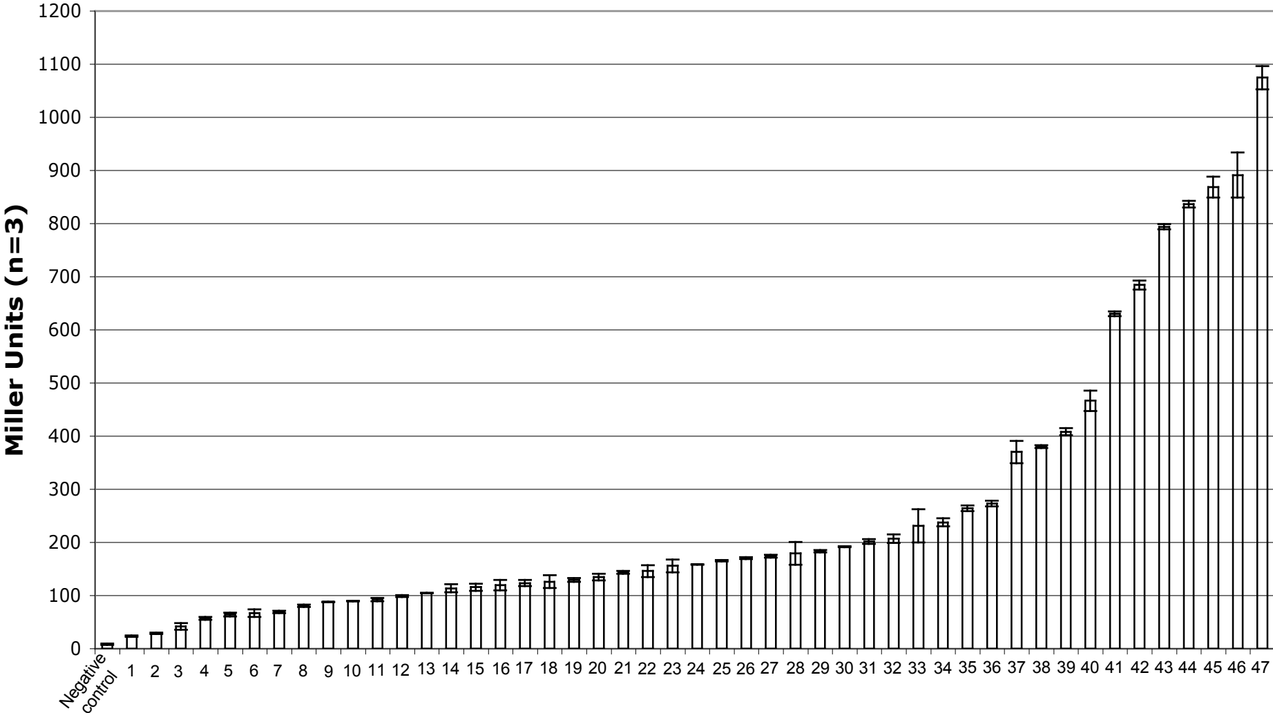
Fig. S1. \beta -Galactosidase activity found with the strains with TnsE-mediated Tn7- lacZ fusions. Strain JP617 was used as the negative control. 47 samples were shown in Figure 6 and other randomly selected isolates from new individual papillation assays. The data shown represent the average of triplicates of each sample. Error bars indicate the standard error of the mean.
