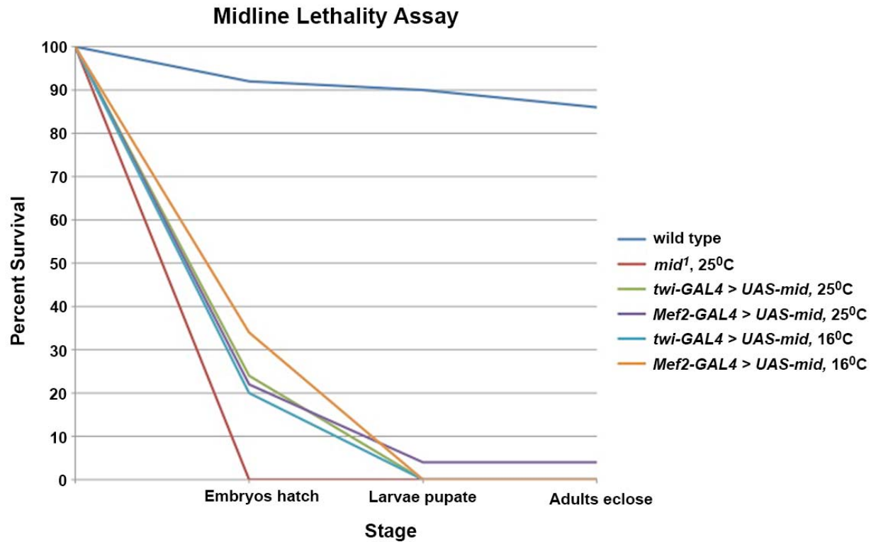
Figure S4 Viability of Midline Loss and Gain. Graph depicting viability of embryos, larvae, pupae and adults of the indicated genotypes, measured as a percent of survivors/total number of embryos selected. Fertilized embryos of the appropriate genotype were hand-selected using fluorescently-marked balancer chromosomes to identify homozygotes. Embryos were then transferred to a plate and monitored for hatching. First instar larvae were then transferred to a vial containing standard cornmeal media for the remainder of the experiment. For all genotypes, n=50.
