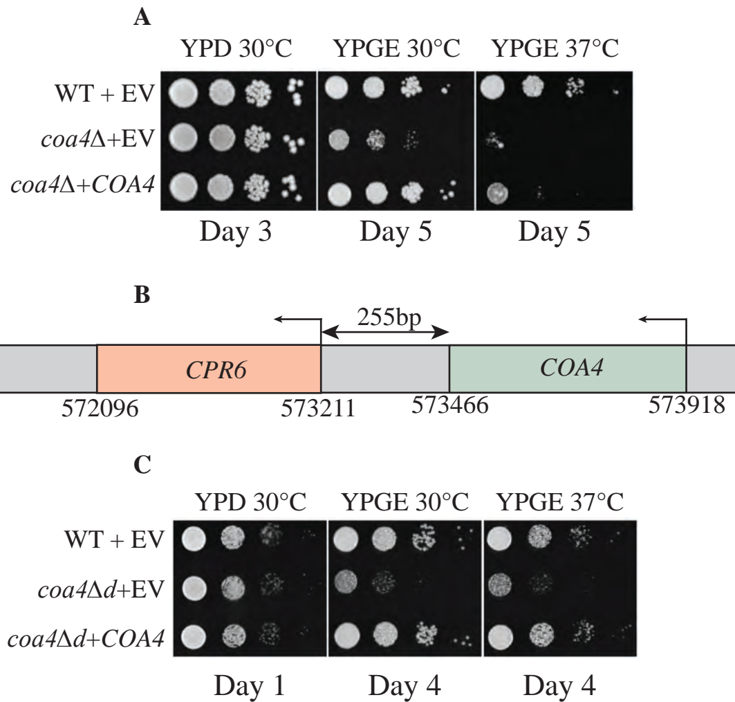
Supplementary figure S3. (A) Ten-fold serial dilutions of the indicated transformants were seeded onto YPD and YPGE plates and were incubated at either 30°C or 37°C. (B) Genome location of CPR6 and COA4 on chromosome XII of yeast. (C) Ten-fold serial dilutions of the indicated transformants were seeded onto YPD and YPGE plates and were incubated at either 30°C or 37°C. Images were taken on the indicated days.
