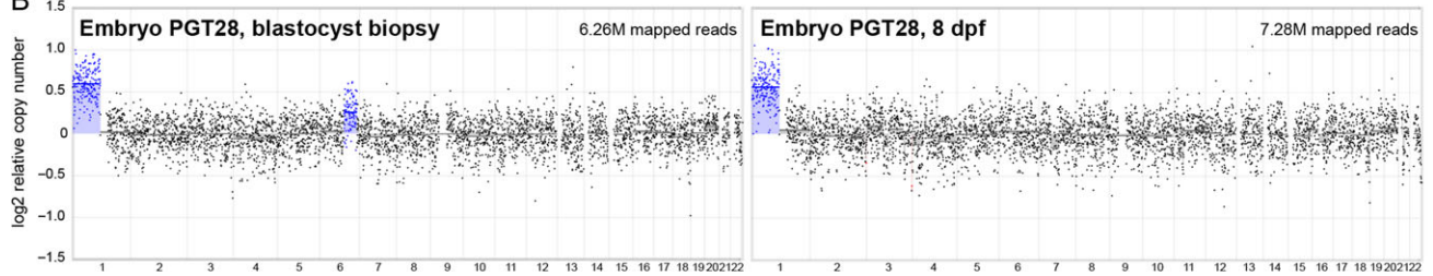
Supplementary Figure S3 Blastocyst diagnosed with chromosomal mosaicism, presented with euploid profiles as early as 8 days post-fertilisation (dpf). M = million (A) Results for embryo PGT22, showing both a mosaic trisomy 1 and mosaic trisomy 16. 1 = Blastocyst profile, 2 = 12 dpf, embryo outgrowth profile. Profiles for both chromosomes 1 and 16, reveal euploid profiles at 8 dpf. (B) Line graph sequencing results for embryo PGT28. The blastocyst biopsy profile revealed a uniform 1.0 log 2 relative copy number in addition to a 55.5 Mb, 6q21q26 mosaic duplication. Only the uniform 118.5 Mb 1p36.33p12 duplication was detected at 8 dpf.
