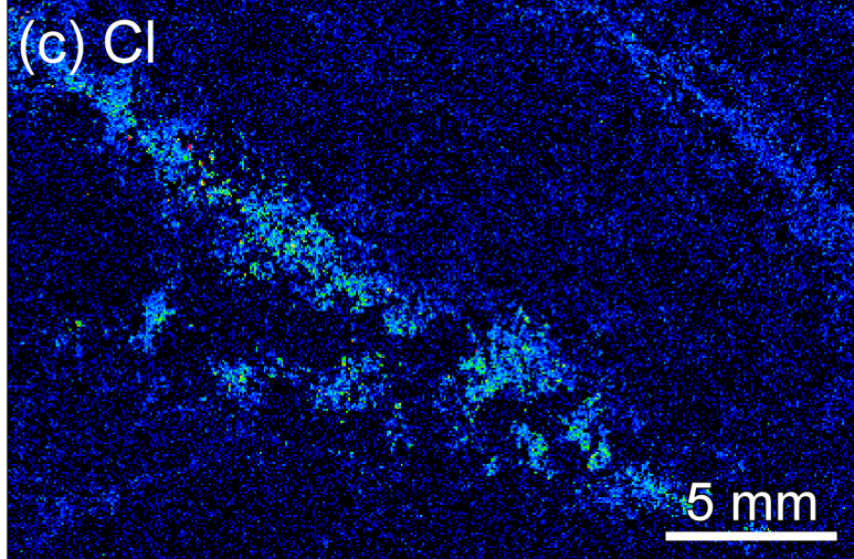
Supplementary Data Electronic Appendix Figure 1. Sample TK2010012403A from Austhamaren. (a) Simplified geological map of the SRM, representing the sample locality. (b) Photo of a whole thin section. Two cracks filled with hornblende discordantly cut the gneissic structure. The yellow boxed area represents the area of an X-ray elemental map in (c). PPL. (c) X-ray elemental map in Cl showing Cl concentration of hornblende grains decreases with distance from the crack. Hornblende in the center of the crack has 0.45 wt% Cl, whereas hornblende in the wall rock has 0.24 wt% Cl.
