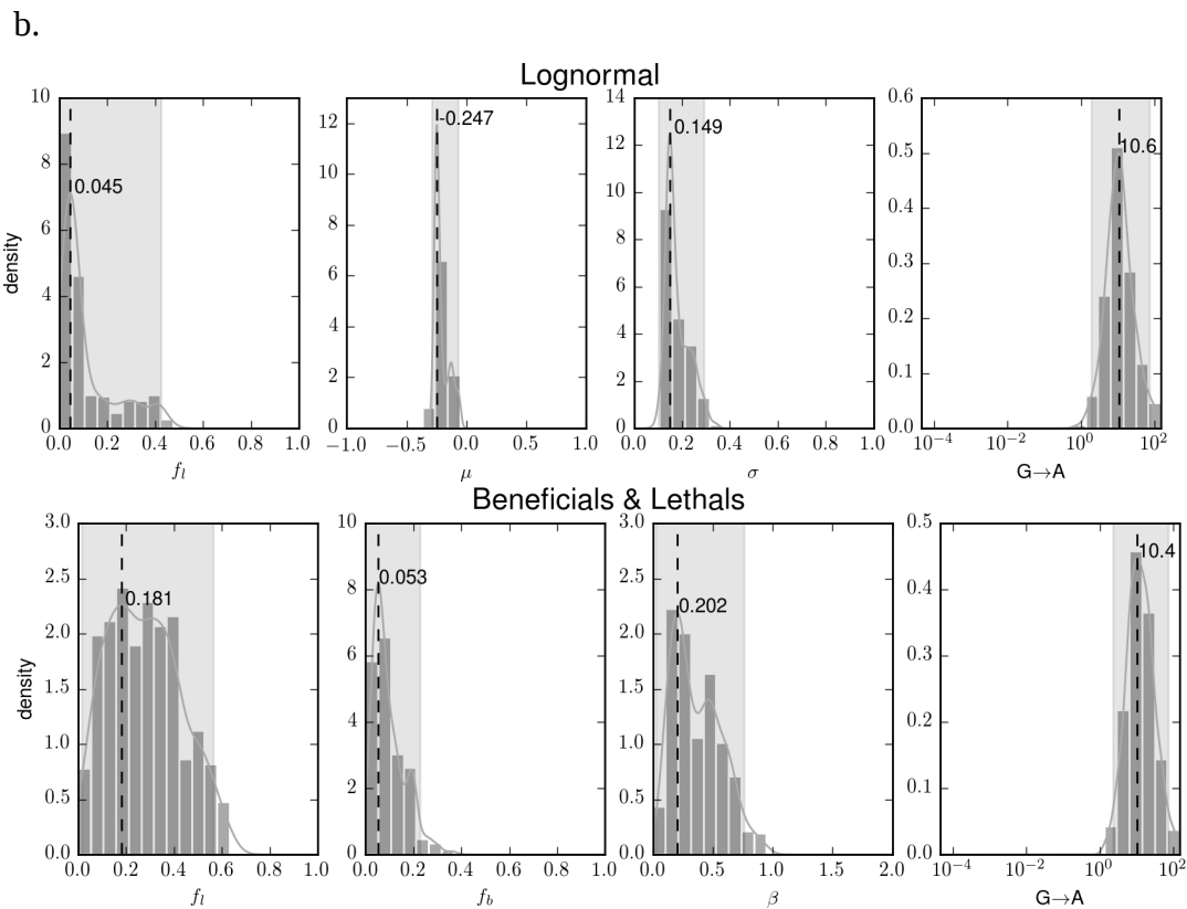
Figure S3: Results of the ABC-SMC fitting procedure. (a) probabilities of the different models S3 across iterations. (b) posterior distribution of the parameters for the lognormal model (top) and ‘beneficials and lethals’ model (bottom). Grey shaded areas indicate the 95% HPD intervals, the black dotted line the highest density point (which is used as the best estimate for the parameters)
