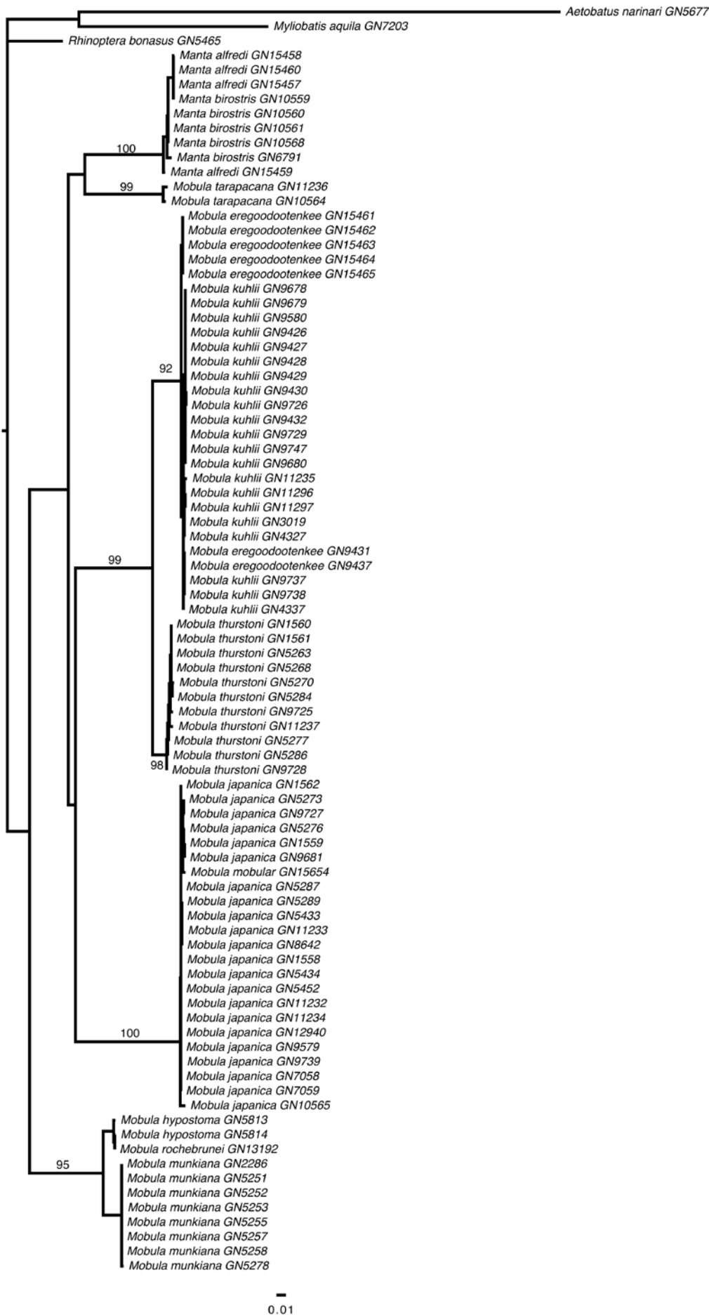
Figure 1. Maximum Likelihood tree showing nominal identifications of mobulid specimens and the relationships among them, relative to three outgroups ( Aetobatus narinari , Myliobatis aquila and Rhinoptera bonasus ). The tree was derived from an alignment of mitochondrial NADH2 sequences (1044 sites) under a TVM+I+G model of molecular evolution.
